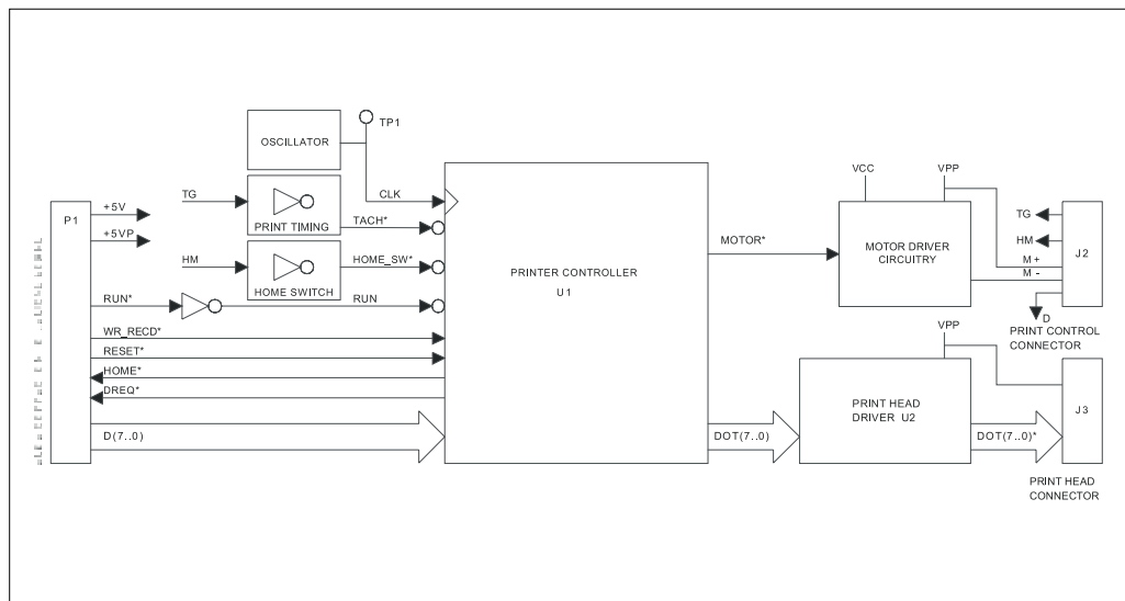
Figure 2-5 Recorder Module Control Logic Block Diagram
