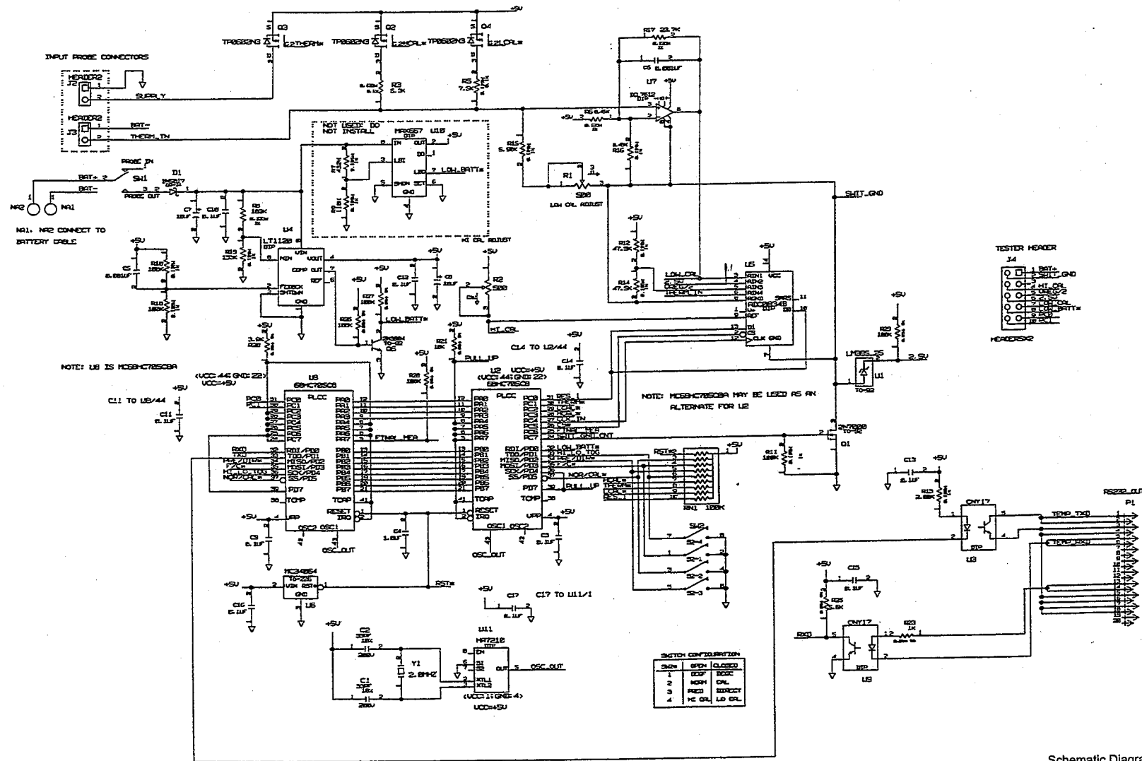
Schematic Diagram Predictive Thermometer Board with Battery 0387-00-0582 Sheet 1 of 1 Revised 12/20/00
