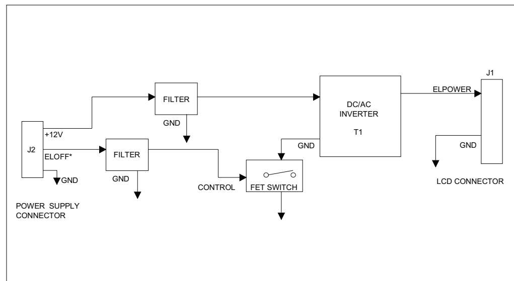
LCD Inverter Module Block Diagram
